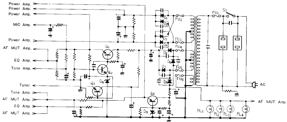
Fig. 8 Power Supply
