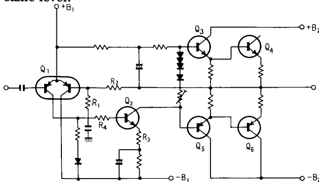
Fig. 7 Power Amplifier
