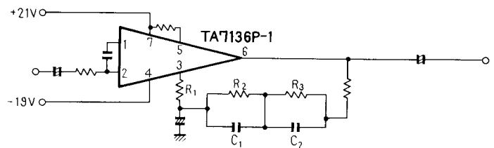
Fig. 2 PHONO Equalizer
