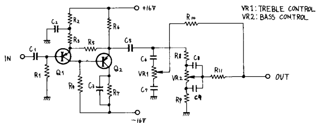
Fig. 4 Tone Control
