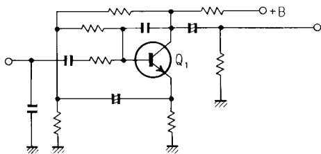
Fig. 3 Microphone Circuit
